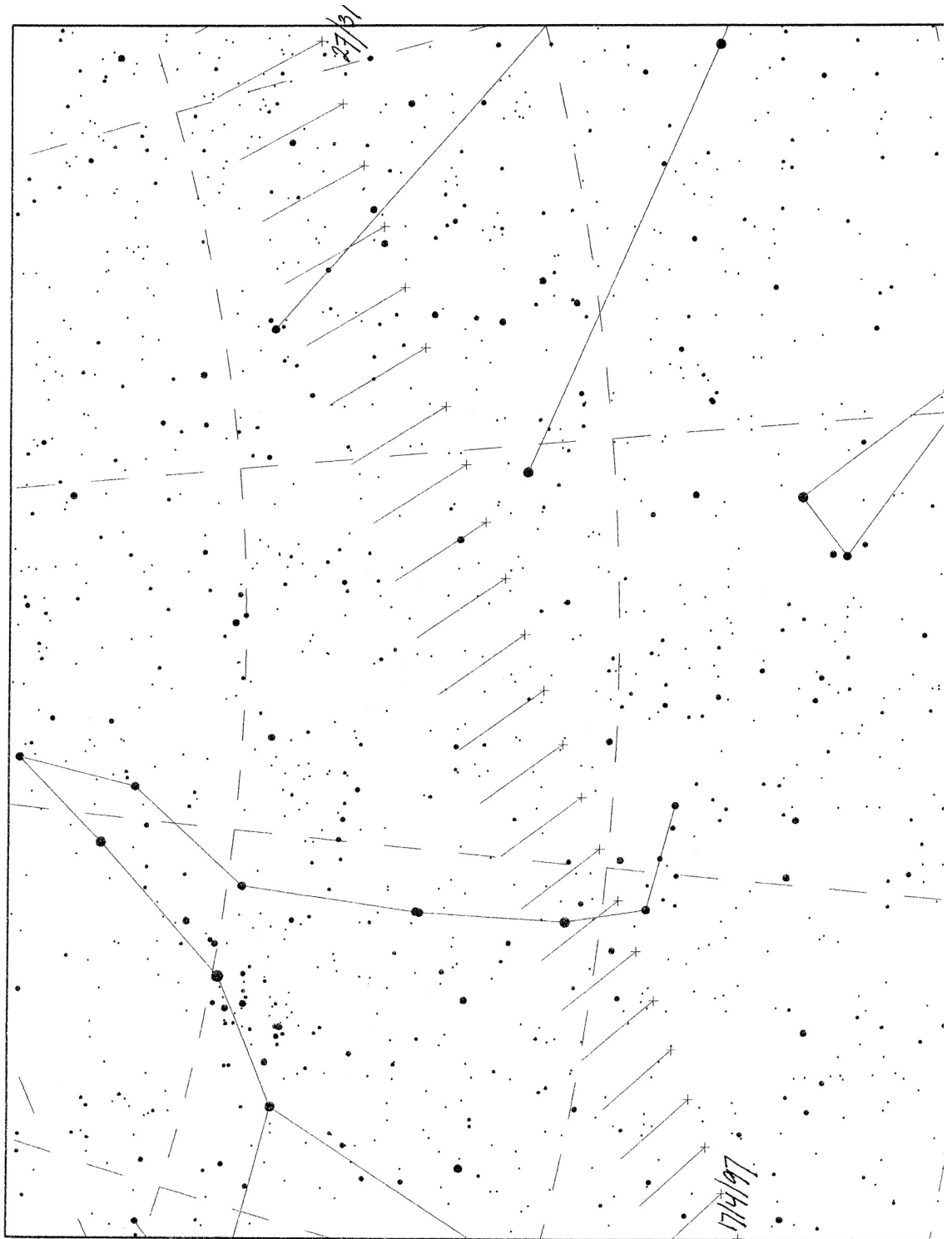
Hale-Bopp positions 2/3/97-17/4/97
