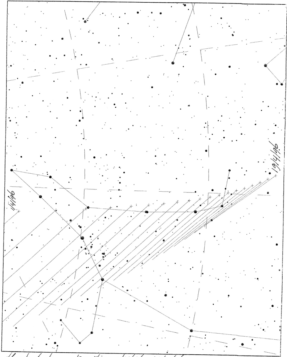
Hyakutake positions 1/4/96-19/4/96
