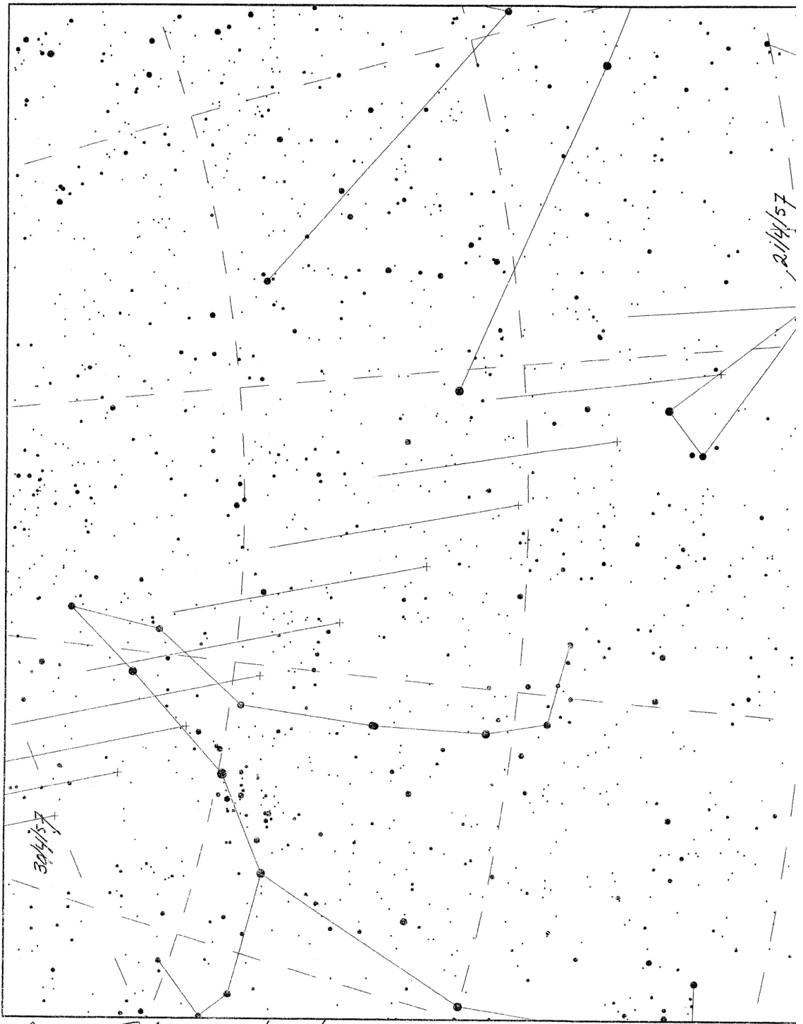
Arend-Roland positions 21/4/57 - 30/4-57
